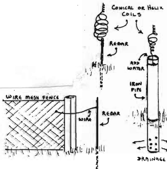
FIGURE 2: ANTENNA SYSTEMS
